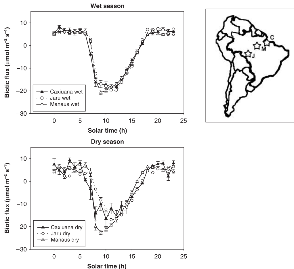
Fig. 2 Fluxes of \text{CO}_2 over three rain forests in Amazonia: Caxiuana (north-east), Manaus (central) and Jarú near Ji Parana (south-west). The fluxes are given as biotic flux (the NEP has been corrected for storage of \text{CO}_2 in the canopy). Sign convention: negative denotes uptake. Each site is represented by data obtained over many days representing the wet and dry seasons. Bars are standard errors. Overall, all three sites show more uptake than loss, i.e. they are carbon sinks. (Reproduced with permission from Andreae et al. 2002.)
