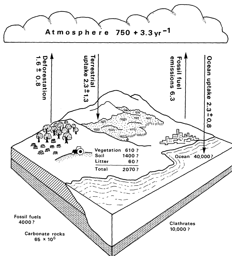
Fig. 1 Carbon sources and sinks. Approximate carbon stocks are shown in units of Gt of carbon; net fluxes are shown by arrows in Gt of carbon per year. Net photosynthesis of the land surface is believed to be made up of about 120 \text{ Gt year}^{-1} of gross photosynthesis and about 60 \text{ Gt year}^{-1} of autotrophic respiration, whilst heterotrophic respiration ('decomposition') is about 60 \text{ Gt year}^{-1} . The sinks shown in the diagram are consistent with inferences from atmospheric concentrations, and calculations referred to later in this article.
